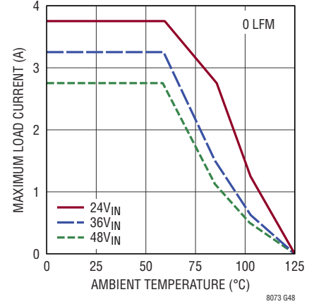
Derating, V_{OUT} = -5\text{V} , BIAS Tied to LTM8073 GND, DC2389A Demo Board
