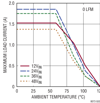
Derating, I-Grade V_{OUT} = -12\text{V} , BIAS Tied to LTM8073 GND, DC2389A Demo Board
